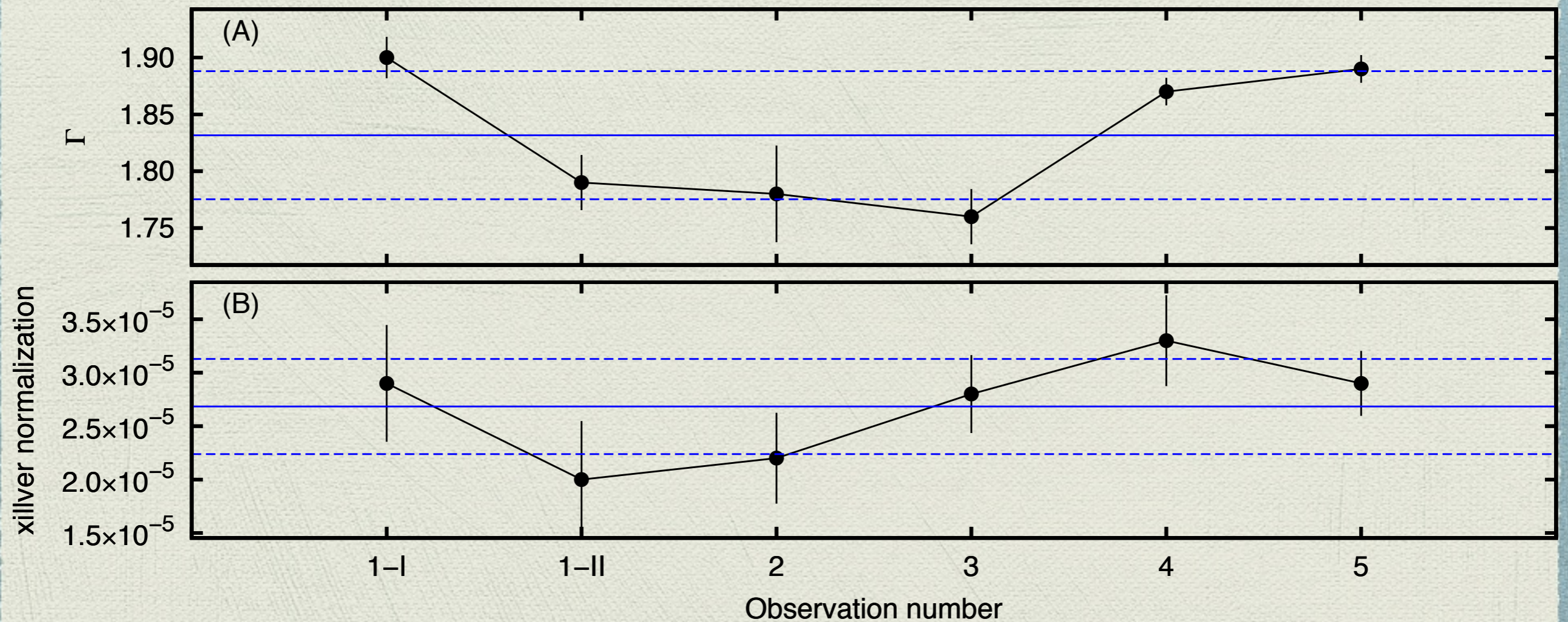
Photon index, xillver normalization
